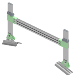
ADJUSTABLE FIBER CEMENT FIXING (1 SIDE)
