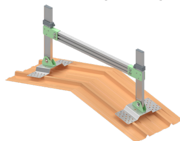
FIBER CEMENT FIXING
